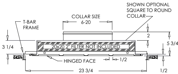
105TFG with square to round collar (optional)
