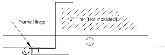
105TFG Frame Detail
