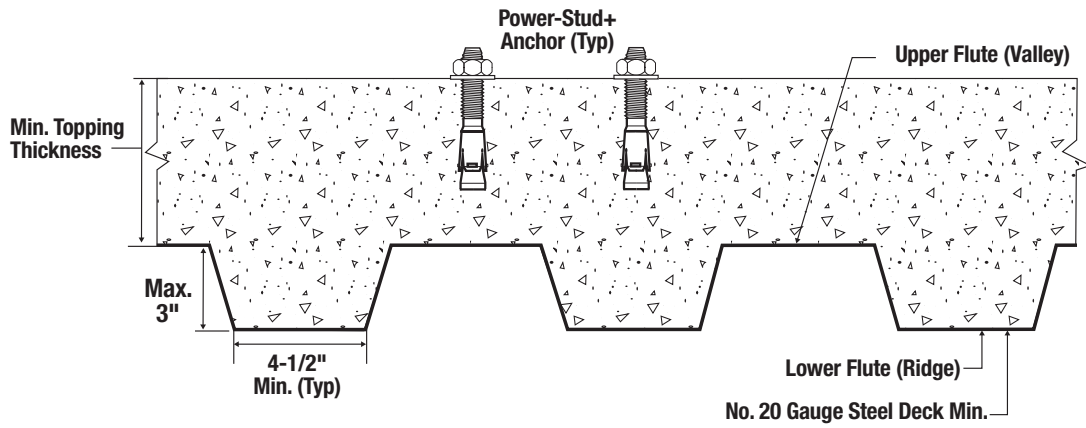
Figure 1B - Power-Stud+ SD1 Installation Detail for Anchors in the Topside of Concrete-Filled Steel Deck Floor and Roof Assemblies (See Dimensional Profile Requirements) 1
